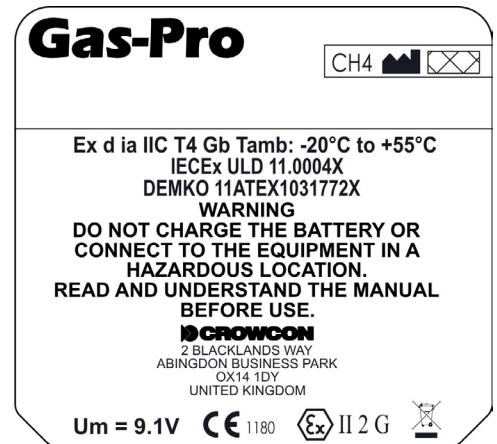
ATEX/IECEX certification label
