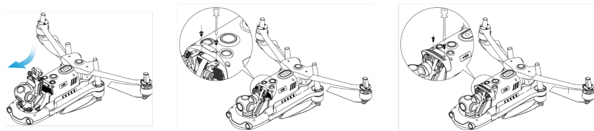
Fig 3-14 Mounting the Gimbal
