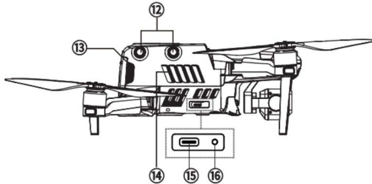
Fig 3-4 Aircraft Right View
