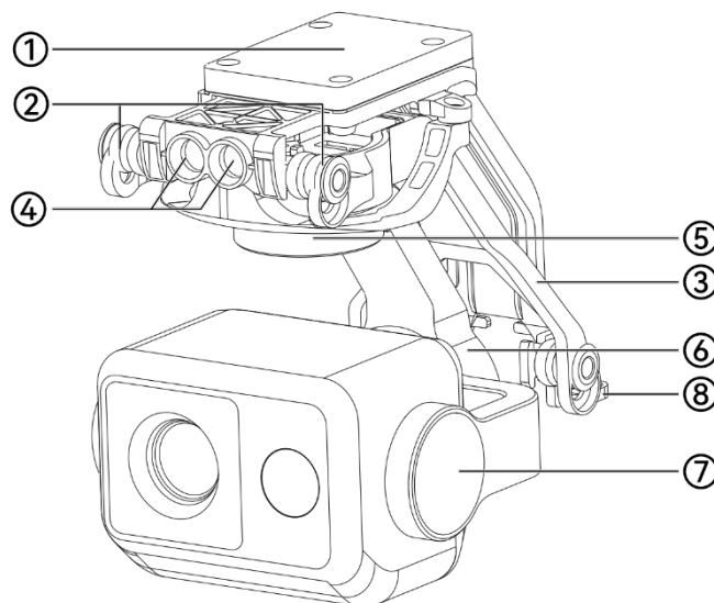
Fig 3-12 Gimbal Structure
