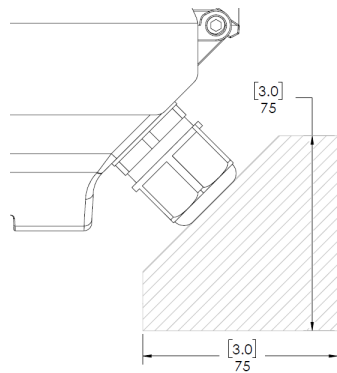
Cable Egress Space (75mm / 3" Bend Radius)
