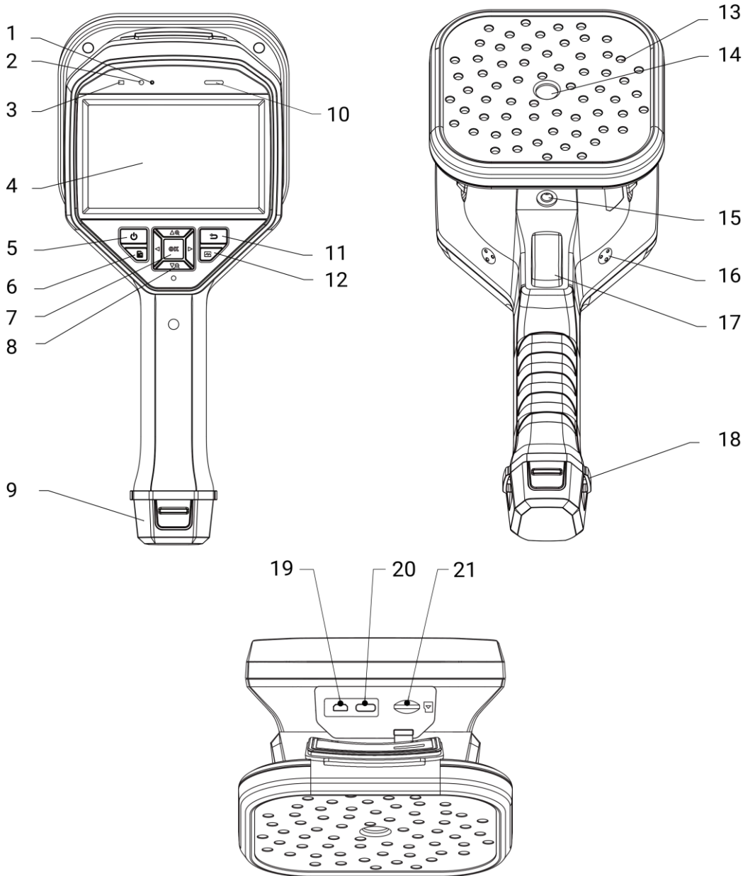
Figure 1-1 Appearance: 64-Microphone Array
