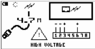
PoE appearing as voltage between pairs 1-2 and 3-6
