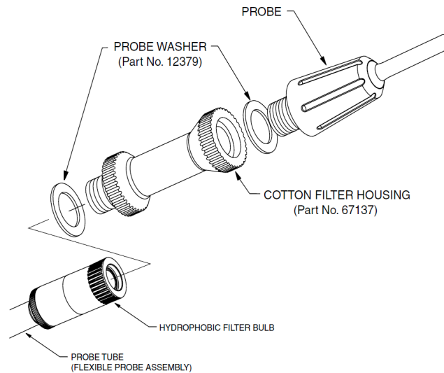
Figure 6-20: Cotton Filter Removal
