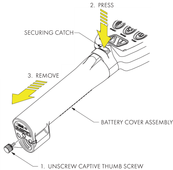
Figure 6-2: Battery Cover Removal
