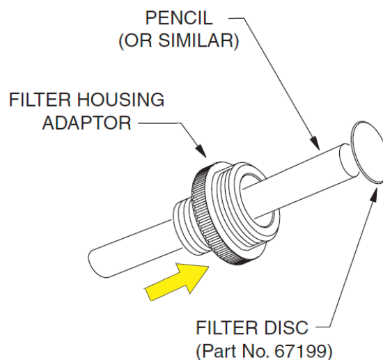
Figure 6-19: Filter Adaptor Removal
