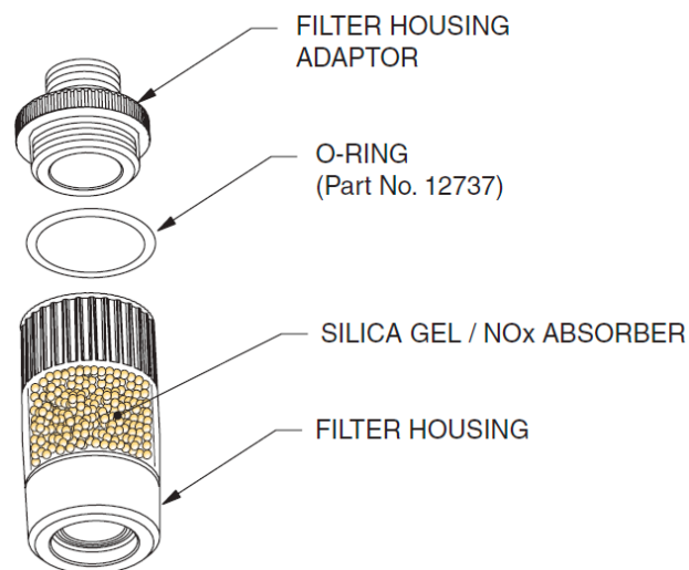
Figure 6-17: Filter Housing Adaptor Removal
