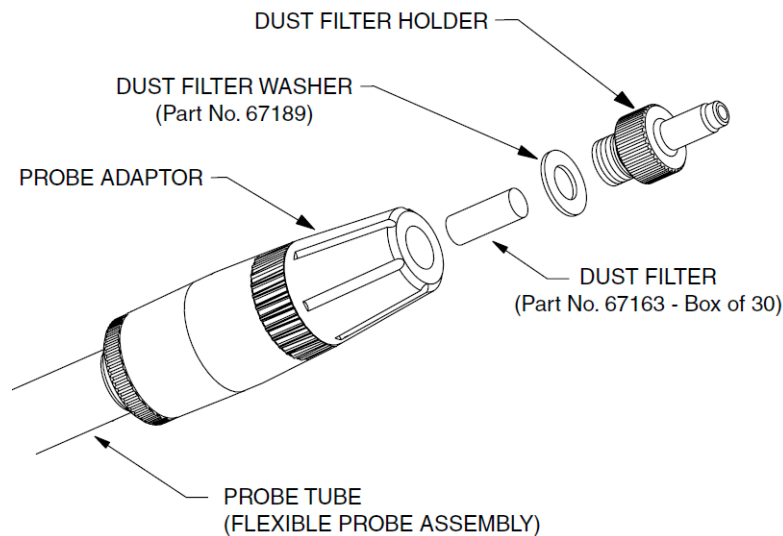
Figure 6-14: Dust Filter Holder / Filter Removal
