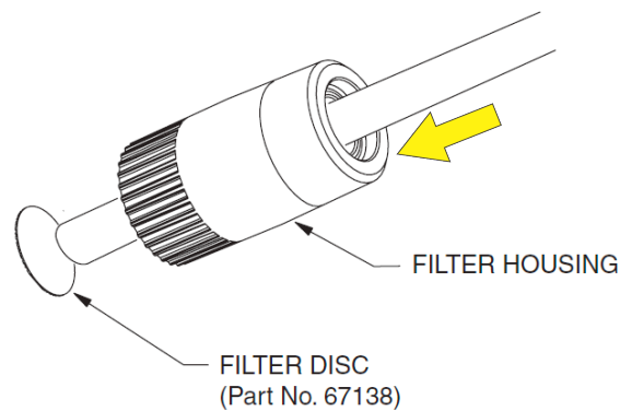
Figure 6-18: Housing Filter Removal
