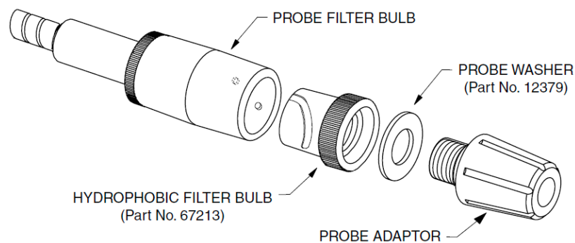
Figure 6-15: Hydrophobic Filter Bulb Removal
