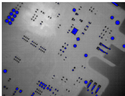
SOLDER POINTS
